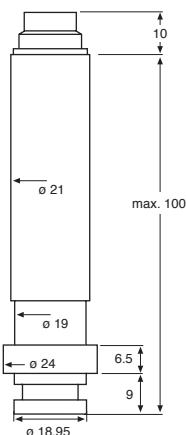
Series 35 X HT (Manometer Pressure Port)
