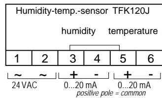
4-wire system (AC-version)
