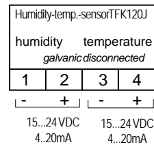
2-wire system
